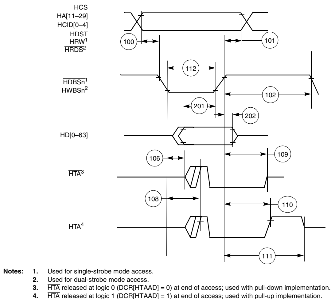
Figure 2-10. Asynchronous Single and Dual Modes Write Timing Diagram
