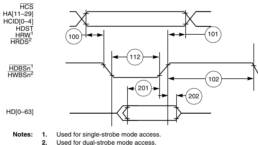
Figure 2-11. Asynchronous Broadcast Write Timing Diagram
